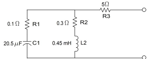
Fig. 8. The impedance model of SP power router.
